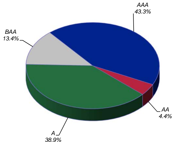
Quality Distribution
