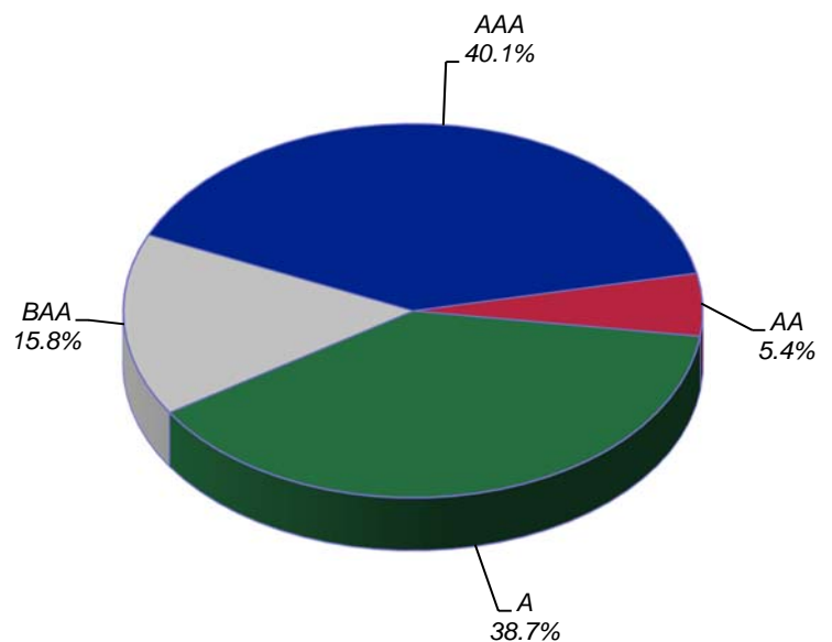
Quality Distribution
