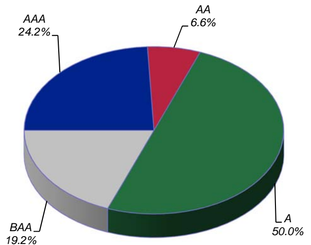
Quality Distribution
