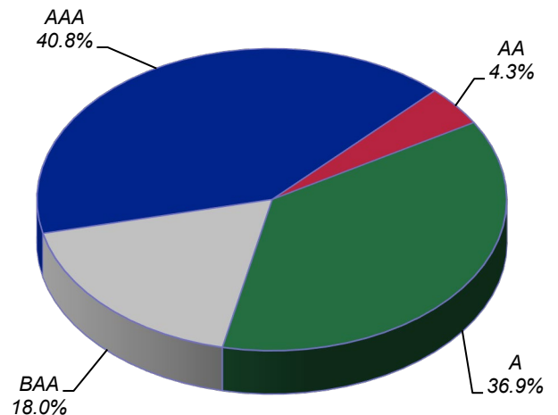
Quality Distribution
